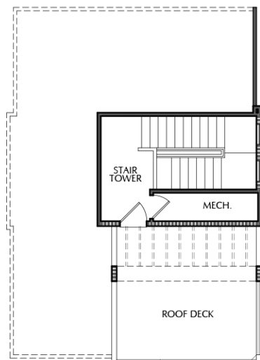
FOURTH FLOOR
